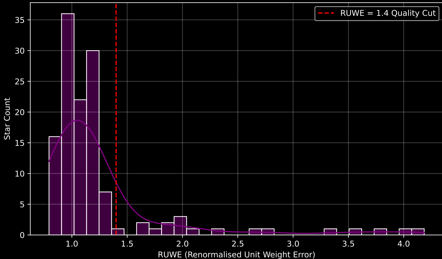
GALAH DR4 Field [7363] RUWE Distribution (n= 129)
