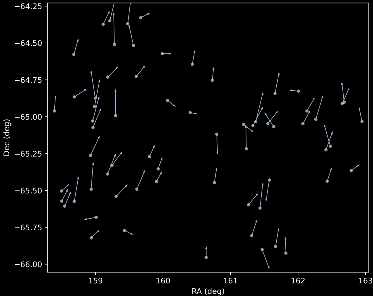
GALAH DR4 Cluster 1 Proper Motion Vectors (n=65)
