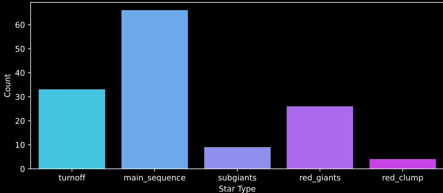
GALAH DR4 Field: [7363] Count plot of Star Type
