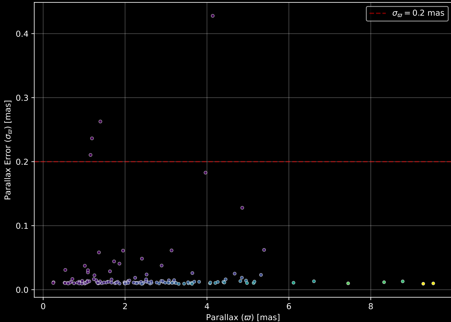
GALAH DR4 Field: [7363] Parallax Quality (n= 138)
