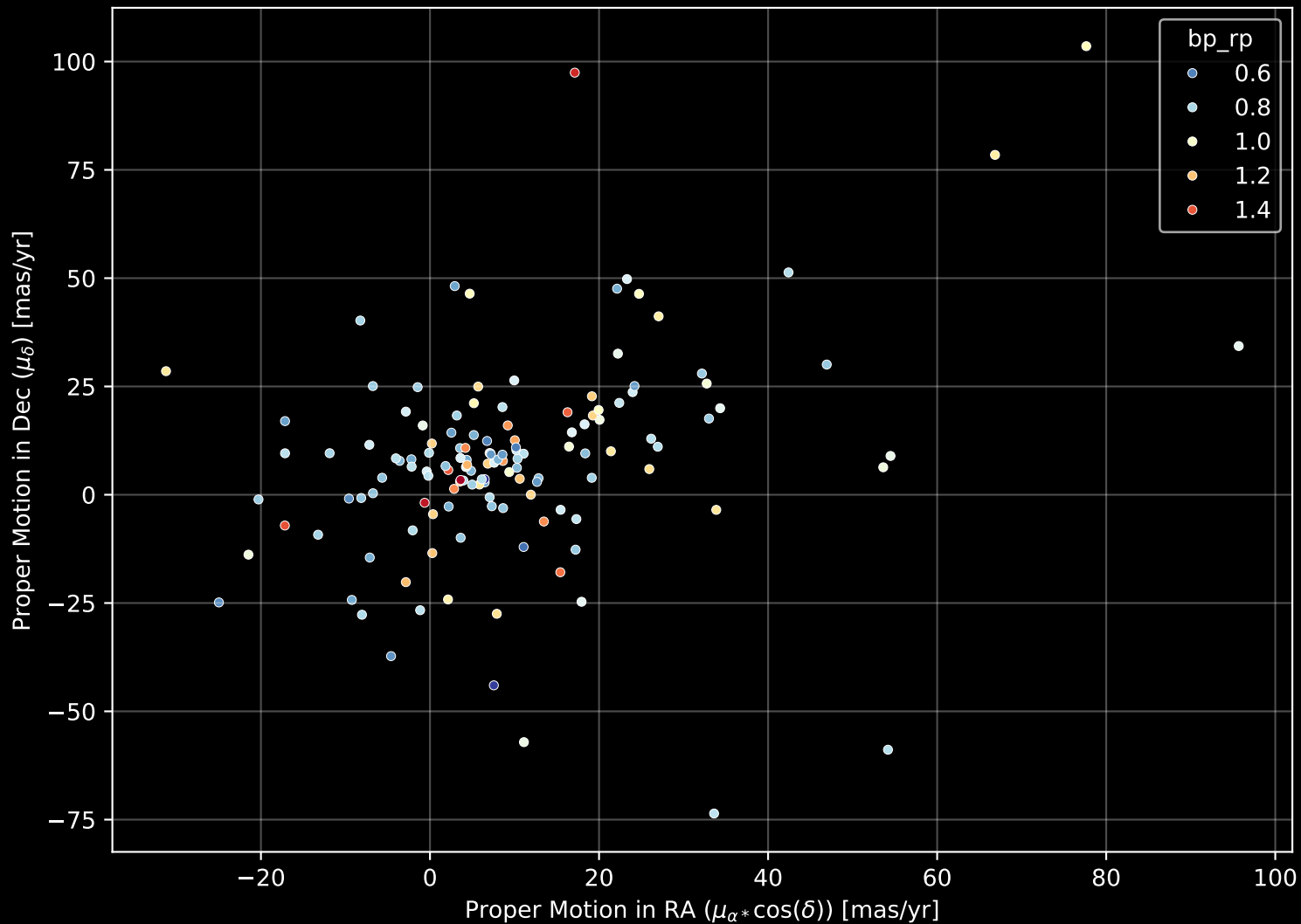
GALAH DR4 Field: [7363] Proper Motion Diagram (n= 138)
